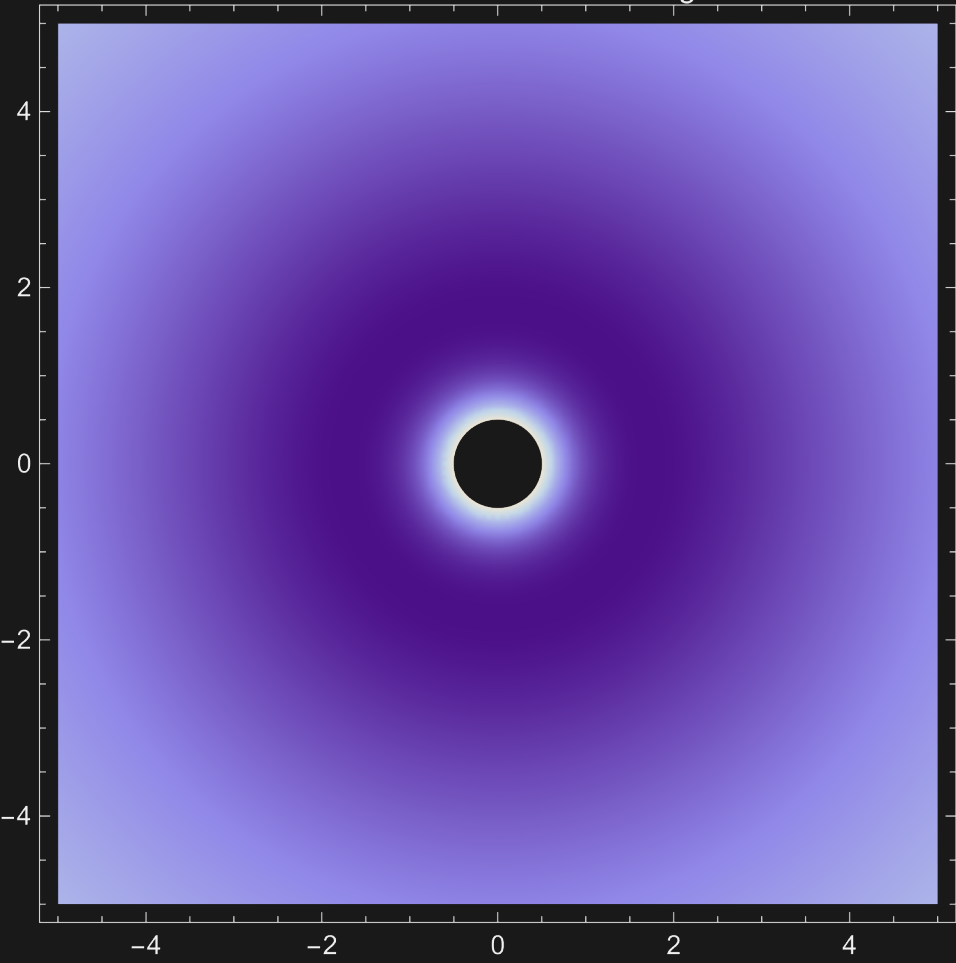
The Grover Horizon: Information Archiving at R=1.15428
